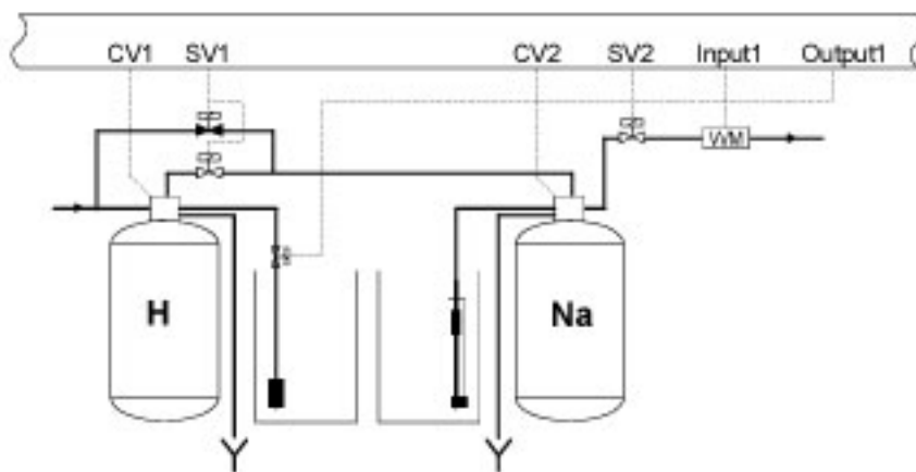
Single run – partial desalination system
