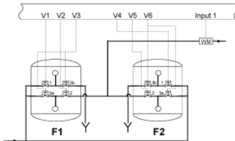
Double sand filter with individual valves.
